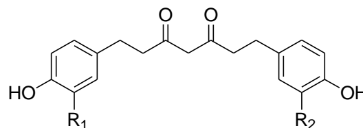
2a , R_1 = R_2 = \text{OCH}_3 2b , R_1 = \text{OCH}_3 , R_2 = \text{H} 2c , R_1 = R_2 = \text{H}
