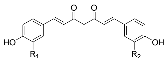
1a , R_1 = R_2 = \text{OCH}_3 1b , R_1 = \text{OCH}_3 , R_2 = \text{H} 1c , R_1 = R_2 = \text{H}
