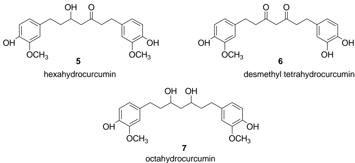
Figure2: Impurities (5-7) formed during synthesis of 2a from 1a
