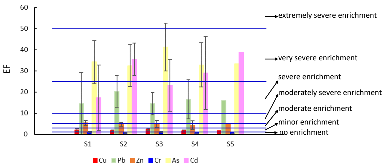
Figure 3. Enrichment factor (EF) of heavy metals in sediment cores of the Cau river
