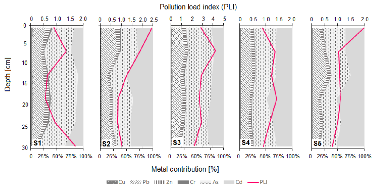
Figure 5. Pollution load indices (PLI) for six heavy metals and their contributions in sediment cores of the Cau river
