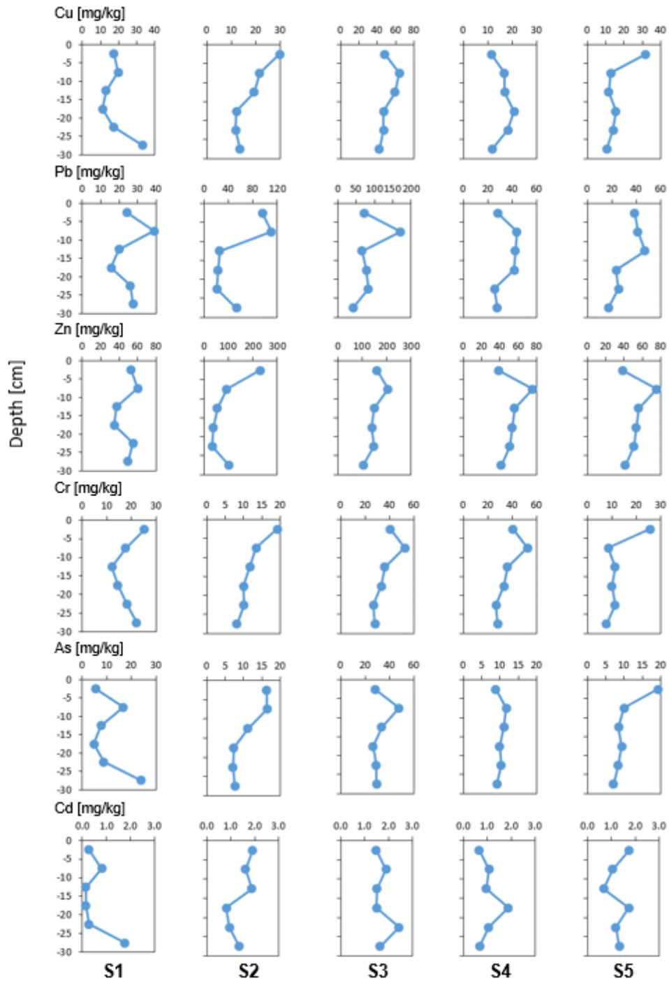
Figure 2. Heavy metal concentration at different sediment depths in the Cau River
