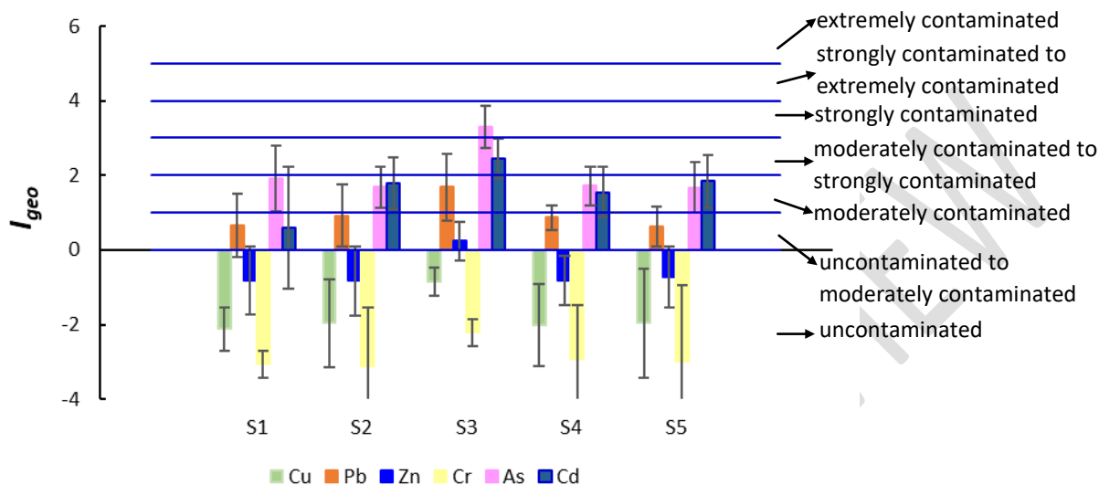
Figure 4. Geo-accumulation index ( I_{geo} ) of heavy metals in sediment cores of the Cau river
