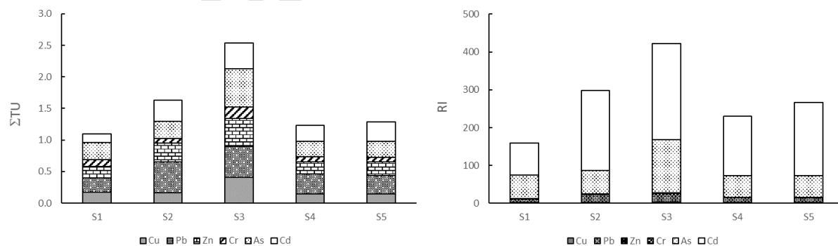
Figure 6. Distribution of the total toxic unit ( \Sigma TU ), and potential ecological risk index (RI) values in sediment cores of the Cau river
