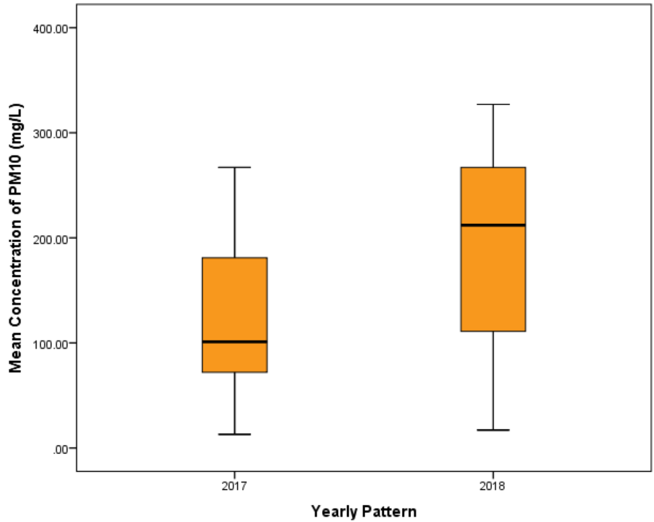
Figure 19: Annual variations in PM 10 concentration between 2017 and 2018 in Port Harcourt, Nigeria
