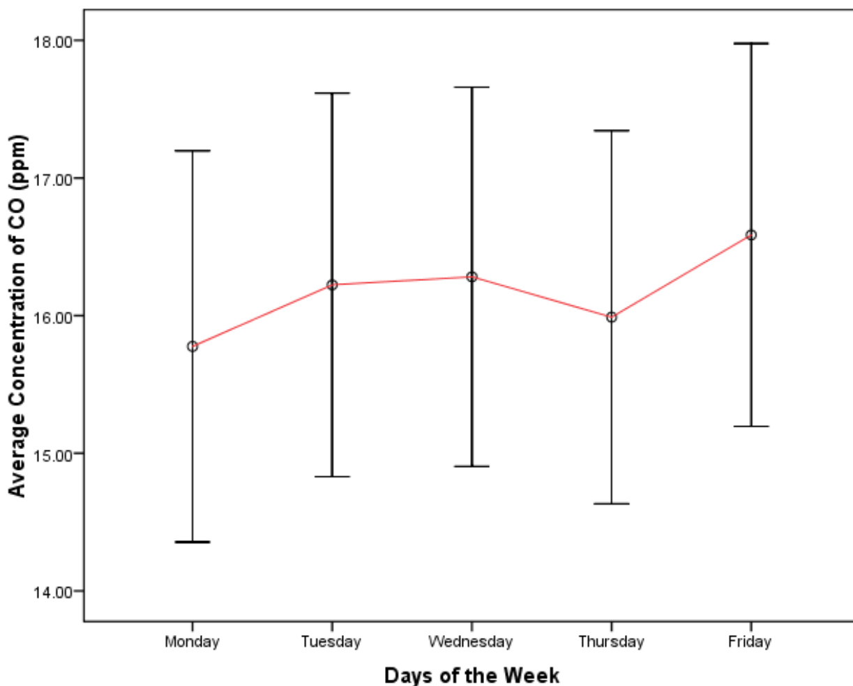
Figure 6: Days of the week variations of CO concentration between 2017 and 2018 in Port Harcourt, Nigeria
