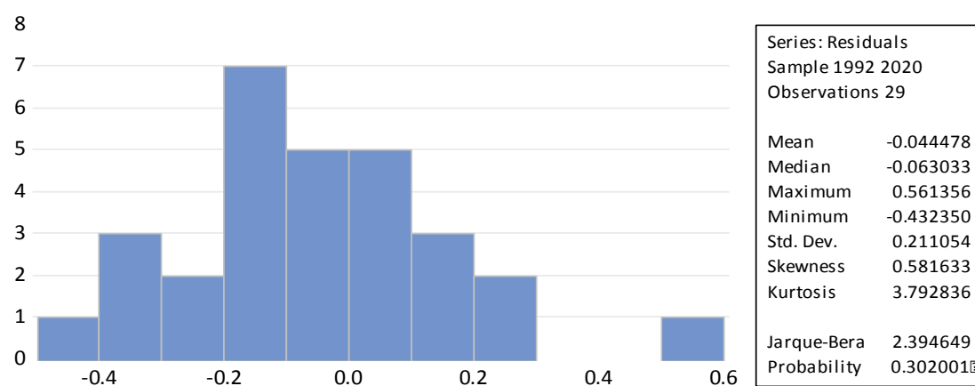
Fig 1: Statistical curve
