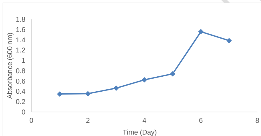
Figure 1: Growth Profile of Bacillus sp on fuel at various time interval
