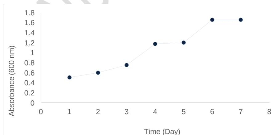
Figure 5: Growth Profile of Bacillus sp on Spent Engine Oil at various time interval
