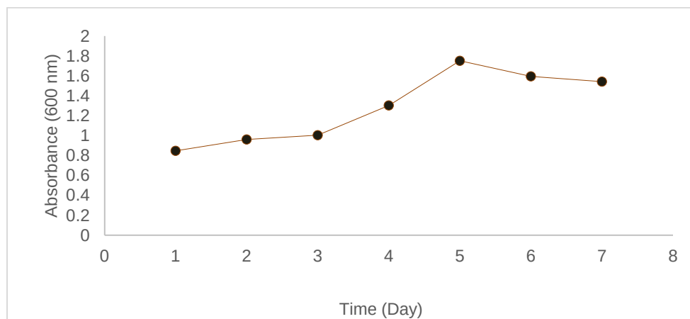
Figure 6: Growth Profile of Staphylococcus sp on Spent Engine Oil at various time interval
