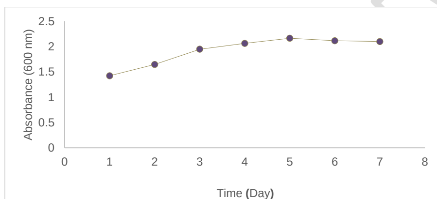
Figure 4: Growth Profile of Staphylococcus sp. on Crude Oil at various time interval
