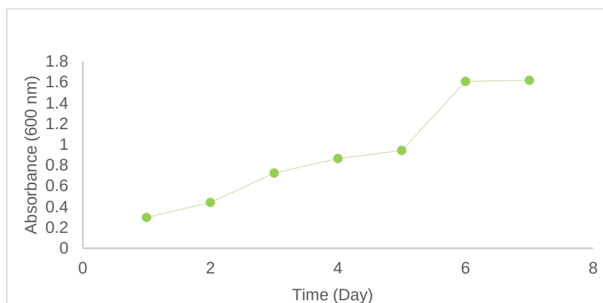
Figure 3: Growth Profile of Bacillus sp. on Crude Oil at various time interval
