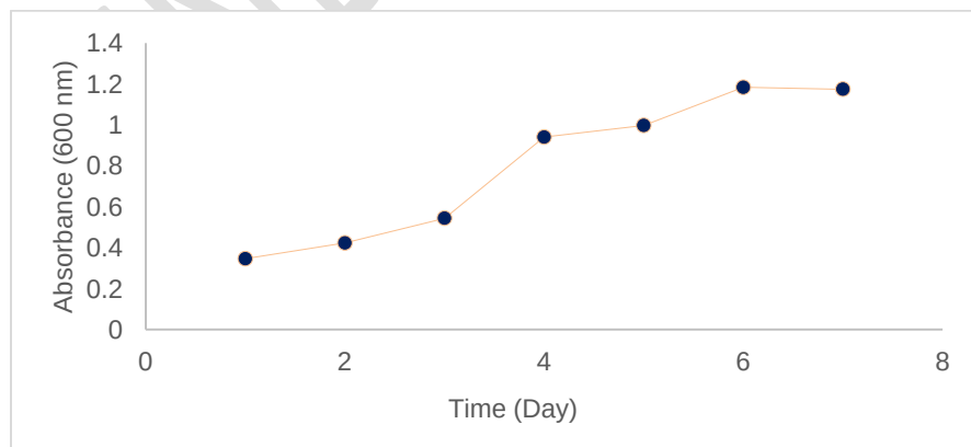
Figure 2: Growth profile of Staphylococcus sp. on Fuel at various time interval
