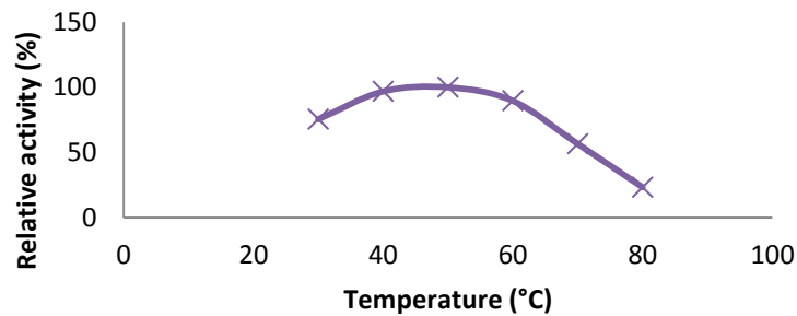
Figure 9: Effect of temperature on activity of purified lipase from Pseudomonas aeruginosa
