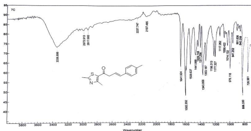
fig-1 (Title?)IR spectrum of thiazolyl styryl ketone
