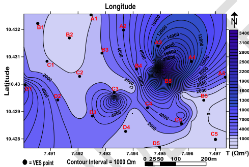
Fig 5: Transverse resistance of the study area.
