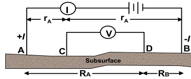
Fig. 2: Schlumberger Configuration for
