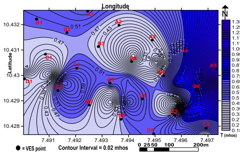
Fig 8: Protective Capacity of the study area.
