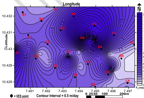
Fig 10: Hydraulic Conductivity of the Area
