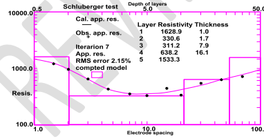
Fig. 3: Typical resistivity curves of VES A2
