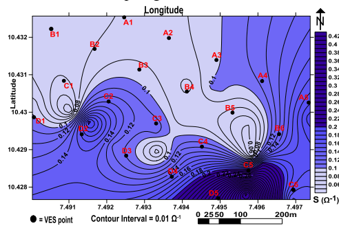
Fig 7: Longitudinal conductance of the area.
