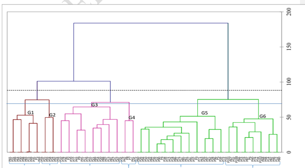
Fig.4. HCA Dendrogram of the coordinates of the readings
