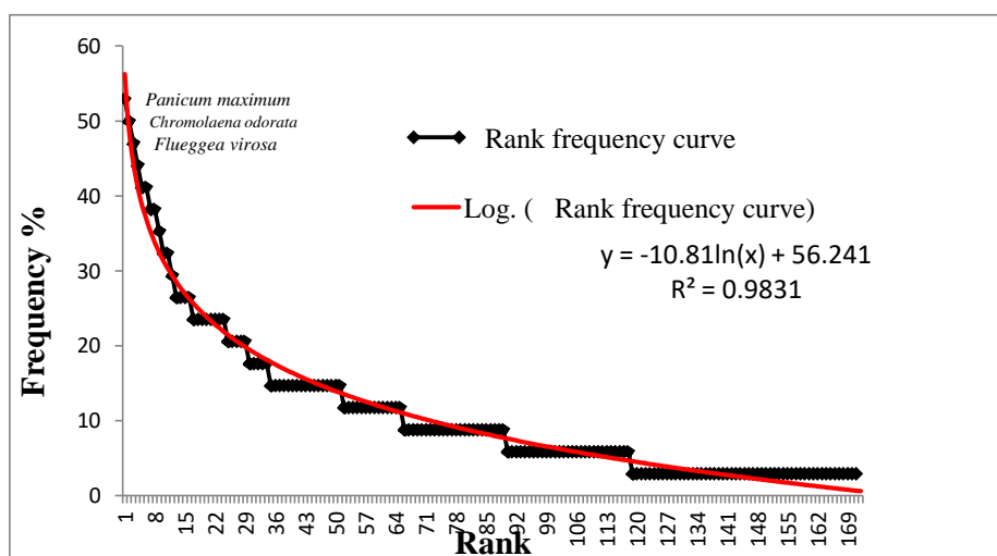
Fig. 2. Distribution species frequencies
