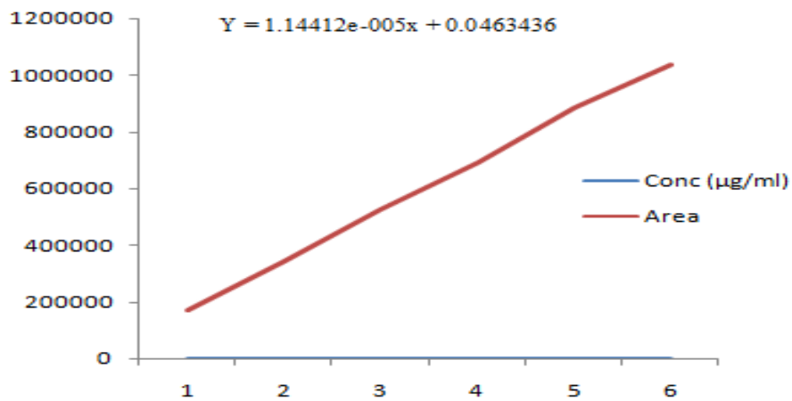
Figure 8: Calibration curve of Empagliflozin
