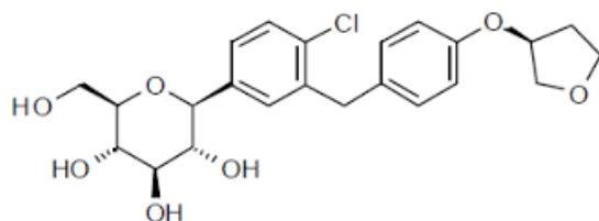
Figure 1. Structure of Empagliflozin
