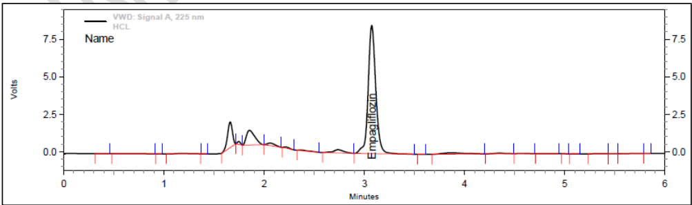
Figure 3: HCl mediated degradation
