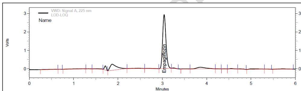
Figure 9: HPLC Chromatogram of standard Empagliflozin
