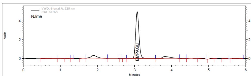
Figure 2: Empagliflozin \lambda_{\text{max}} at 225 nm in methanol
