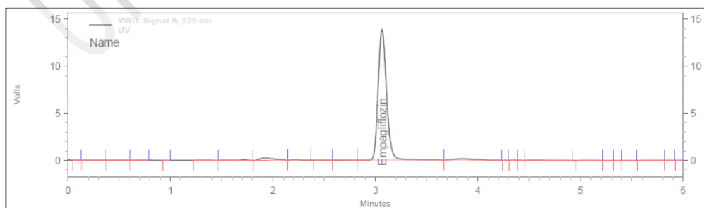
Figure 7: UV Light degradation
