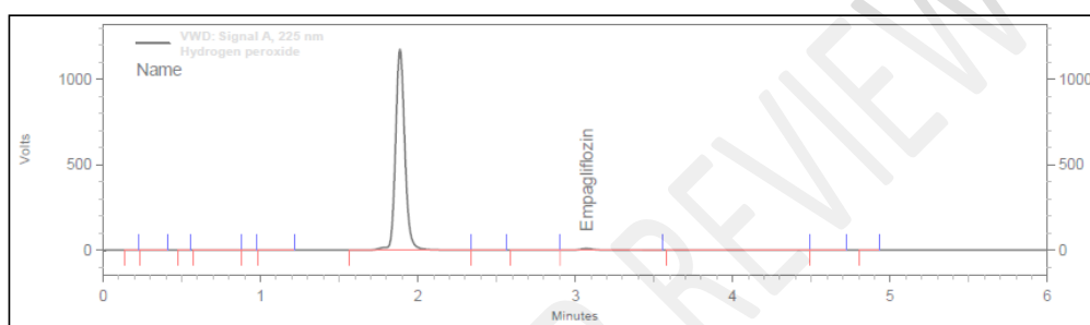
Figure 5: Hydrogen peroxide mediated degradation
