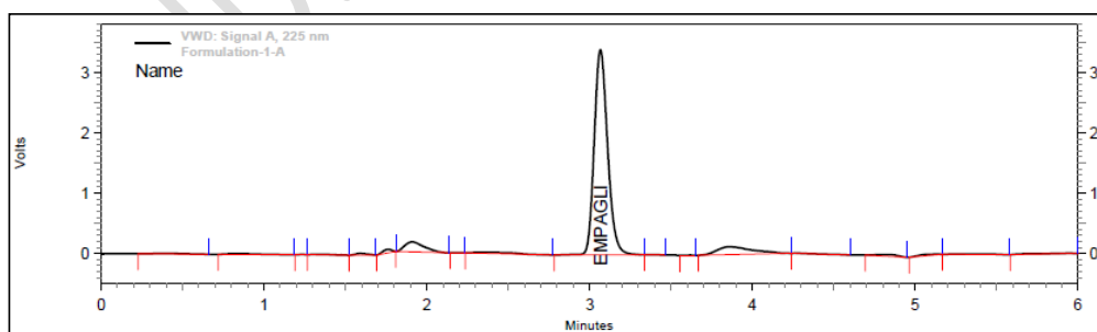
Figure 10: HPLC Chromatogram of Brand 1
