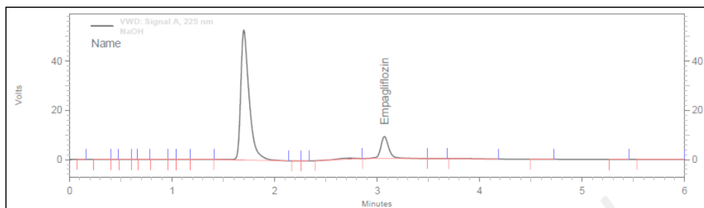
Figure 4: NaOH mediated degradation
