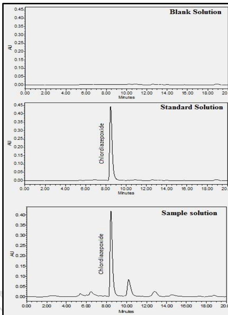
Figure 1: Chromatograms for Blank, Standard and Sample
