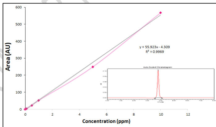
Figure 1. Calibration curve of BRX (HPLC)
