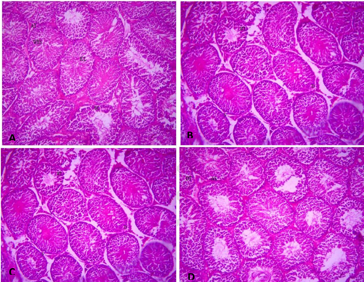
Figure 1 : Representative Photomicrograph of rat testis: A (control) shows normal testicular architecture with active seminiferous tubules that are lined with interstitial cells of Leydig (ICL), Sertoli cell (SC) and well enhanced spermatogenesis (ES); B (rats exposed to 30°C warm water) shows mild distortion (D) of the seminiferous tubules otherwise normal with moderately enhanced spermatogenesis (S); C (rats exposed to 35°C warm water) shows normal seminiferous tubules with mild focal area hemorrhage (H) within the basal layer; D (rats exposed to 40°C warm water) shows seminiferous tubules with moderate arrest of the spermatogenesis (AS) and areas of cellular distortion. (H/E) (x400).
