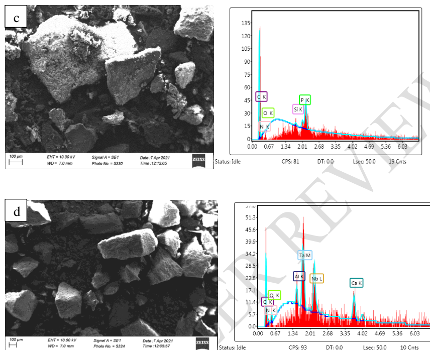
Fig 2. SEM/EDX results at EHT = 10.00kv and wavelength of 100 \mu m for a.) Isiagu Clay sample b.) Chicken droppingsand c.) Melon Shell d.) Palm Kernel Shell
