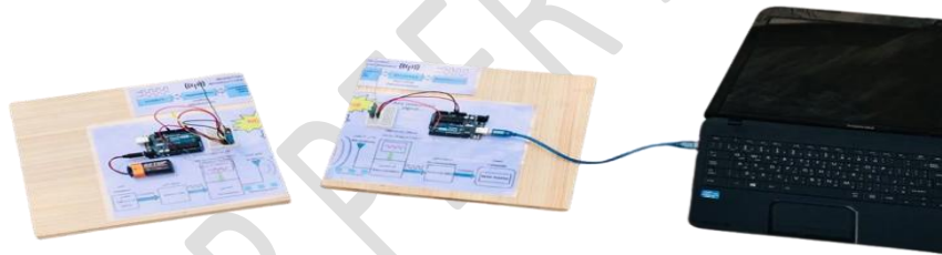
Figure 9. The full system of transmitting and receiving digital information wirelessly at 433MHz
