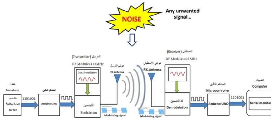
Figure 4. Proposed system.
