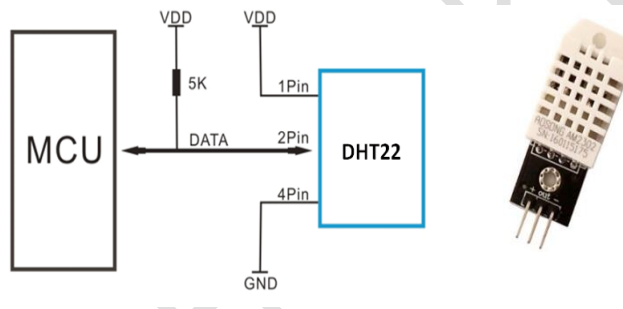
Figure 1. DHT22 temperature and humidity sensor
