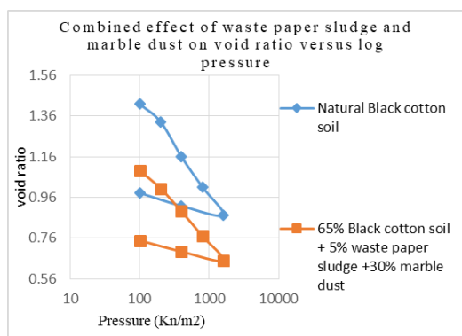
Figure 4 Combined effects of Waste paper sludge and Marble dust on Void Ratio Versus Log Pressure with Loading and Unloading for Test Pit 2
