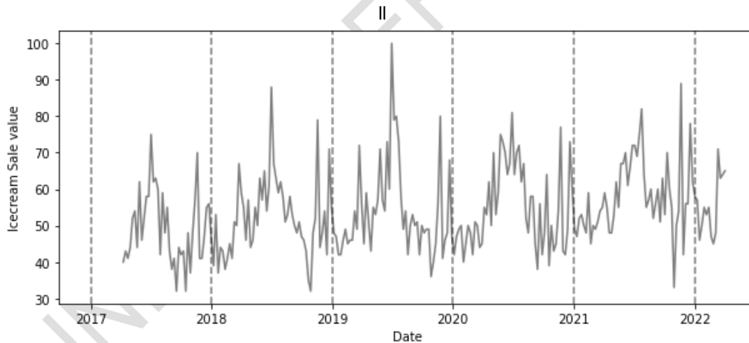
Fig. 2. Visualization of Ice cream data
