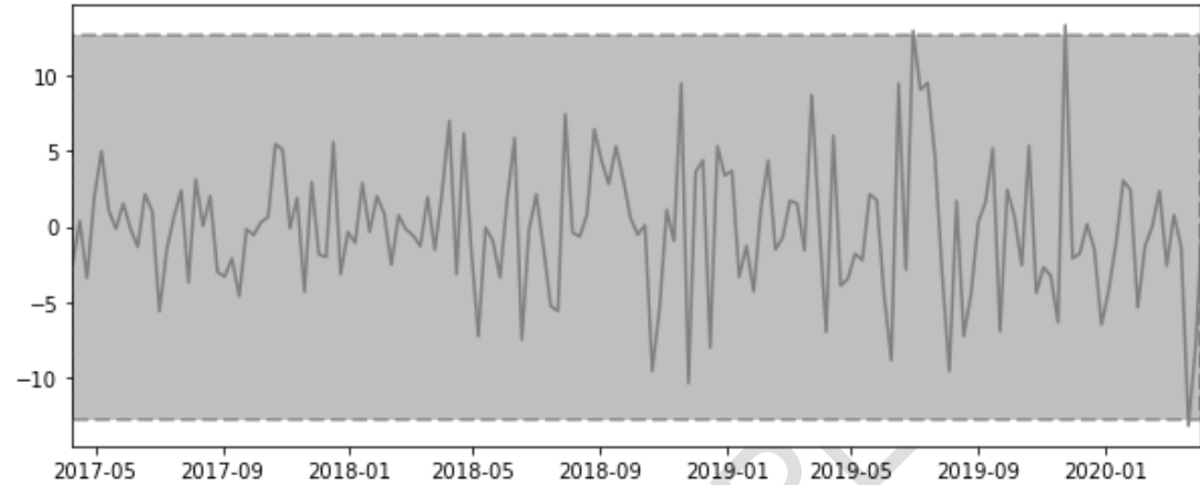
Fig. 5. Isolating abnormal points from the residual data
