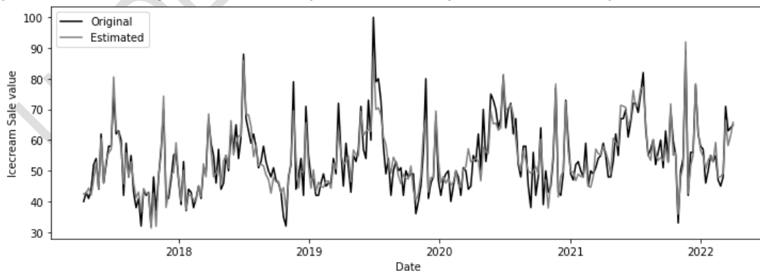
Fig. 4. The original and the estimated points for the Ice cream sales data
