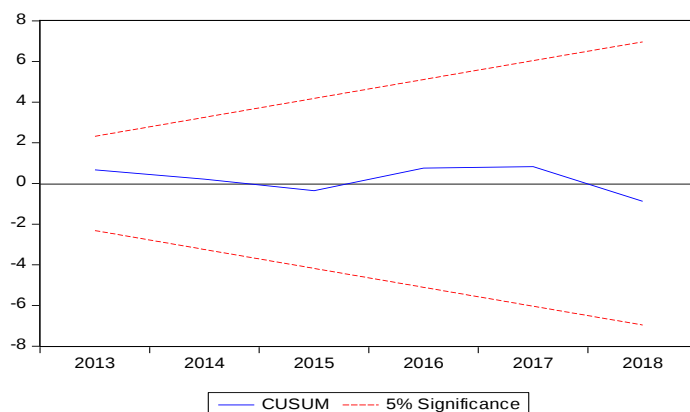
Fig. 6. CUSUM test of diagnostic stability
