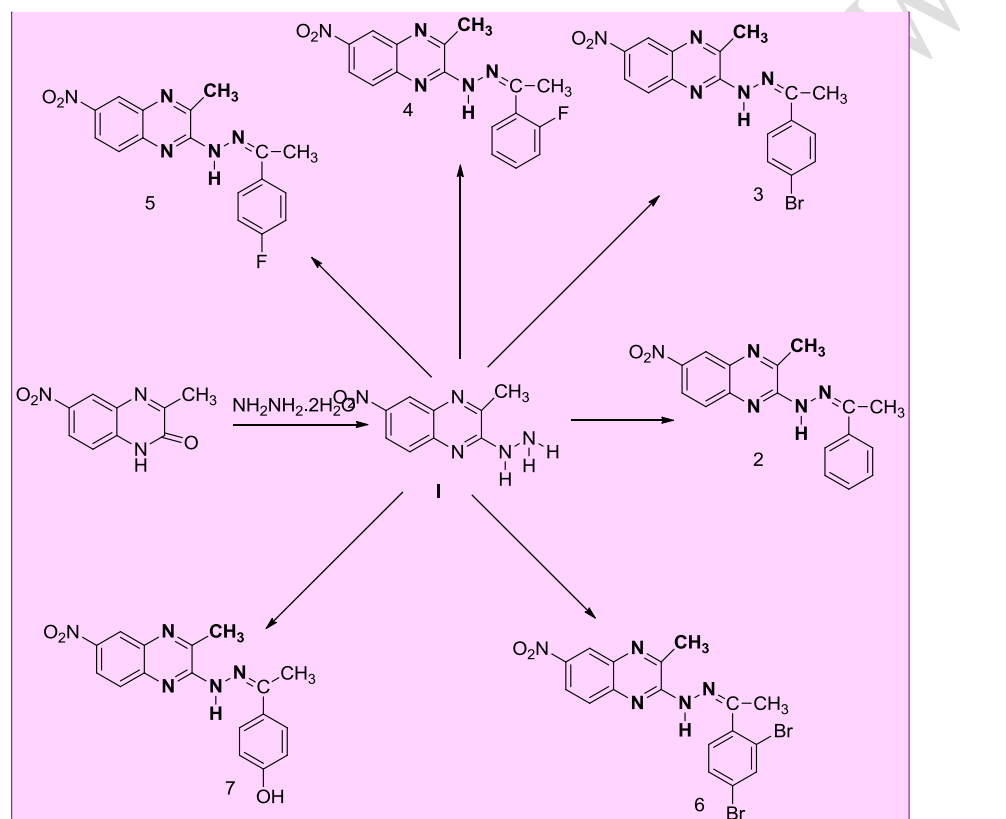
Scheme 1: Reaction of 3-methylquinoxalin-2-hydrazine (I) with various substituted acetophenones
