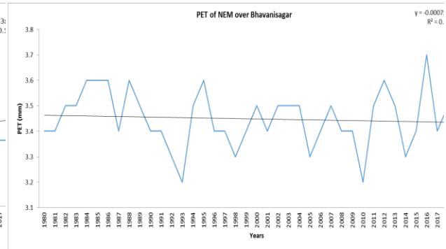
Fig 3. PET of NEM over Bhavanisagar
