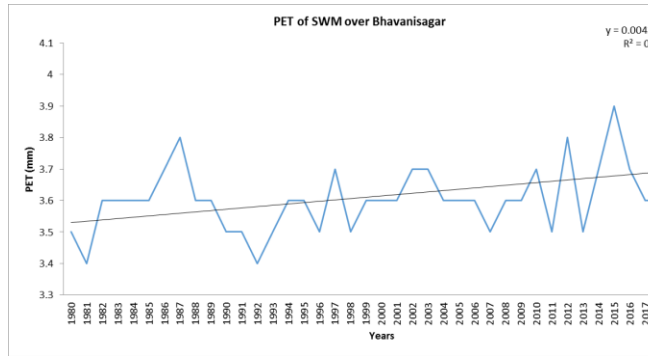
Fig 2. PET of SWM over Bhavanisagar
