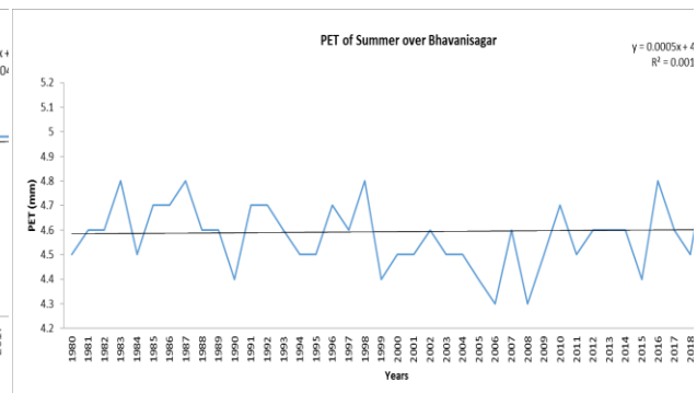
Fig 5. PET of Summer Season over Bhavanisagar
