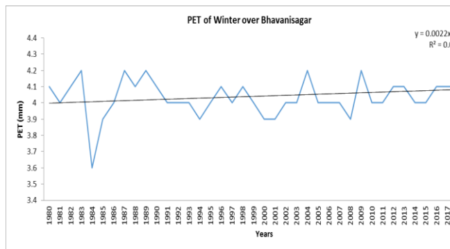
Fig 4. PET of Winter Season over Bhavanisagar
