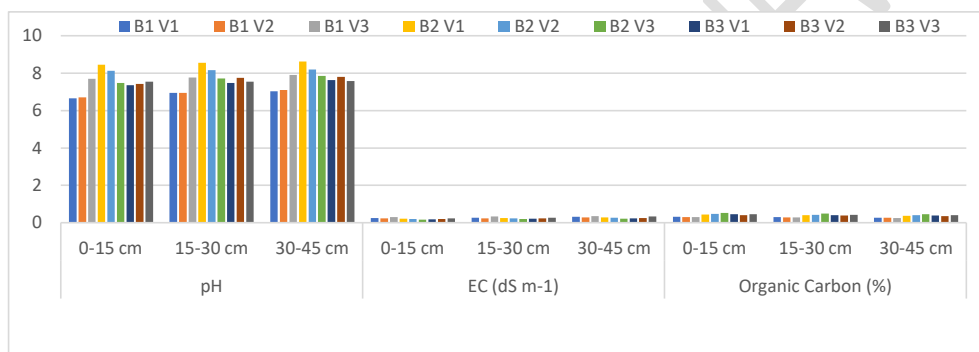
Fig 2: Graphical representation of pH, EC (dS m -1 ), Organic Carbon (%)
