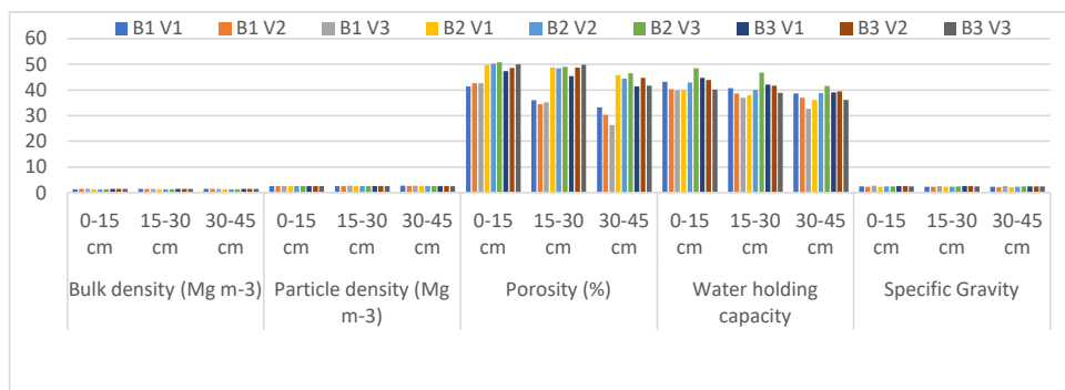
Fig 1: Bulk density (Mg m -3 ), Particle density (Mg m -3 ), Porosity (%), WHC (%) and Specific gravity are all represented graphically
