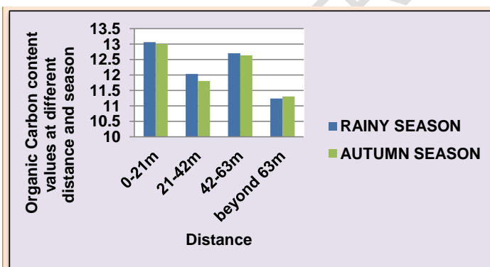
Fig. 5.2:- Organic Carbon content ( \text{g kg}^{-1} ) at different distances and season
