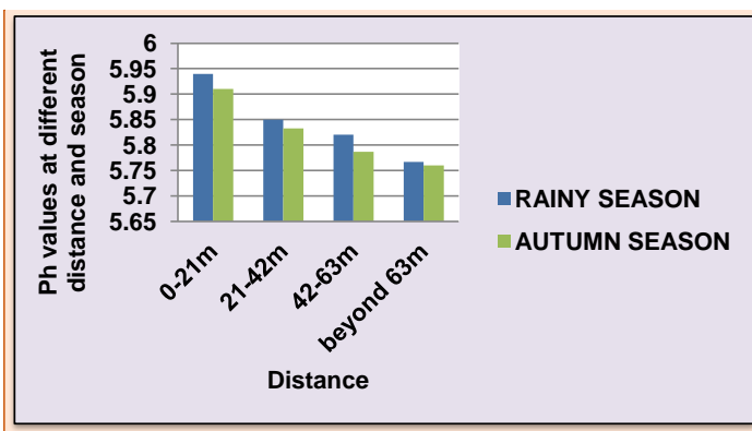
Fig. 5.1:- Ph at different distances and season
