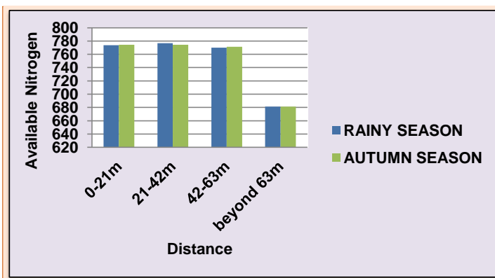
Fig. 6.1:- Available Nitrogen ( \text{kg ha}^{-1} ) at different distances and season
