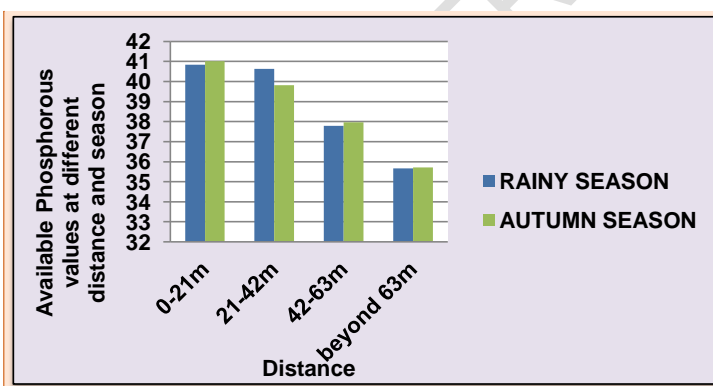
Fig. 6.2:- Available Phosphorous ( \text{kg ha}^{-1} ) at different distances and season
