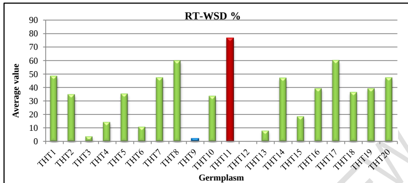
Fig. 8. Variation in RT-WSD % of different germplasm
