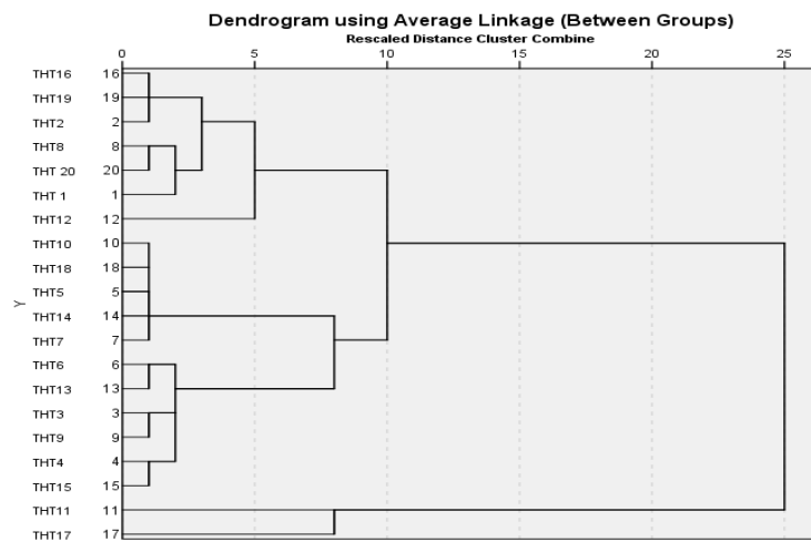
Fig. 11. Dendrogram base on abiotic parameters
