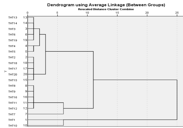
Fig. 7. Dendrogram done by using pigment characters
