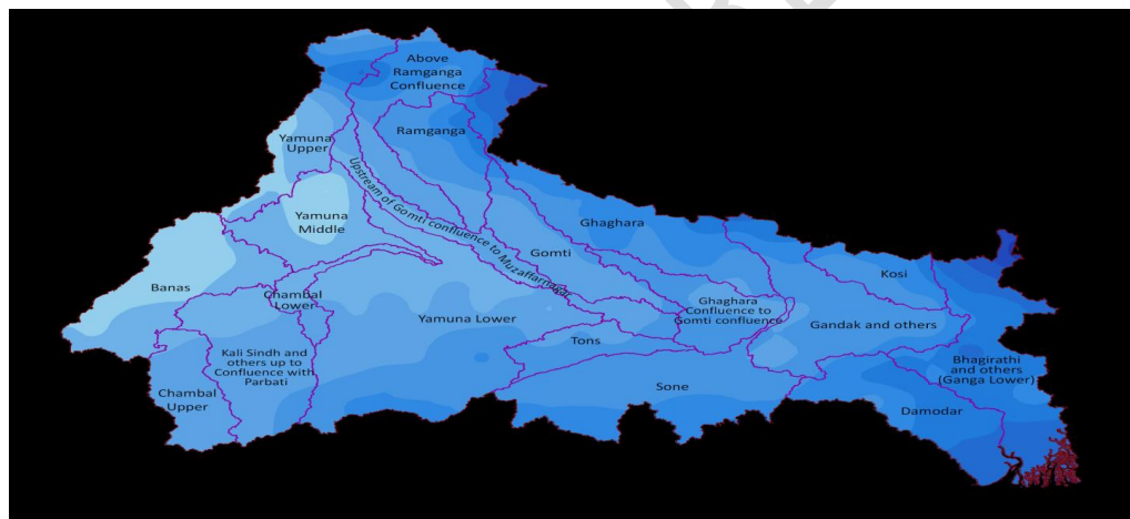
Fig 5. Average annual rainfall (1971-2005)
