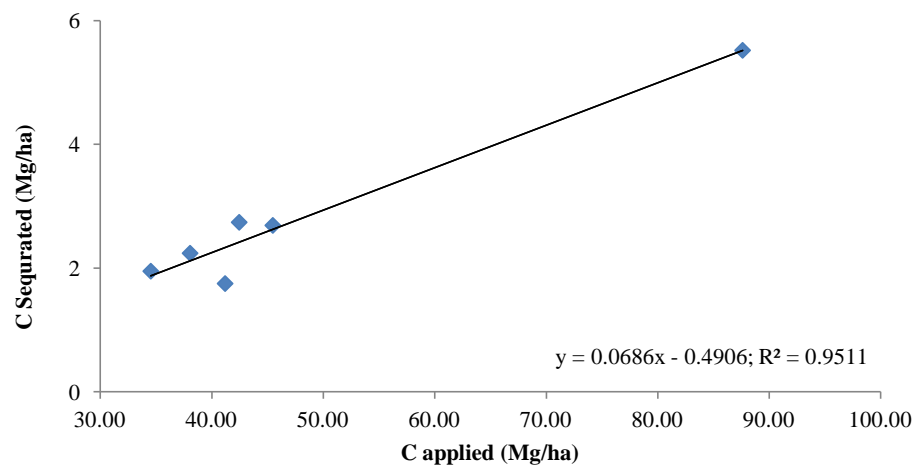
Fig 1: Relationship between cumulative C input and C sequestration and critical value for zero change in total organic carbon (TOC) stock
