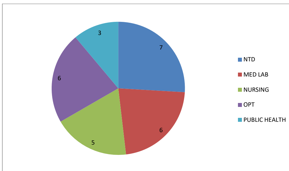
Figure 1: A pie chart showing the departmental base prevalence of the pathogens
