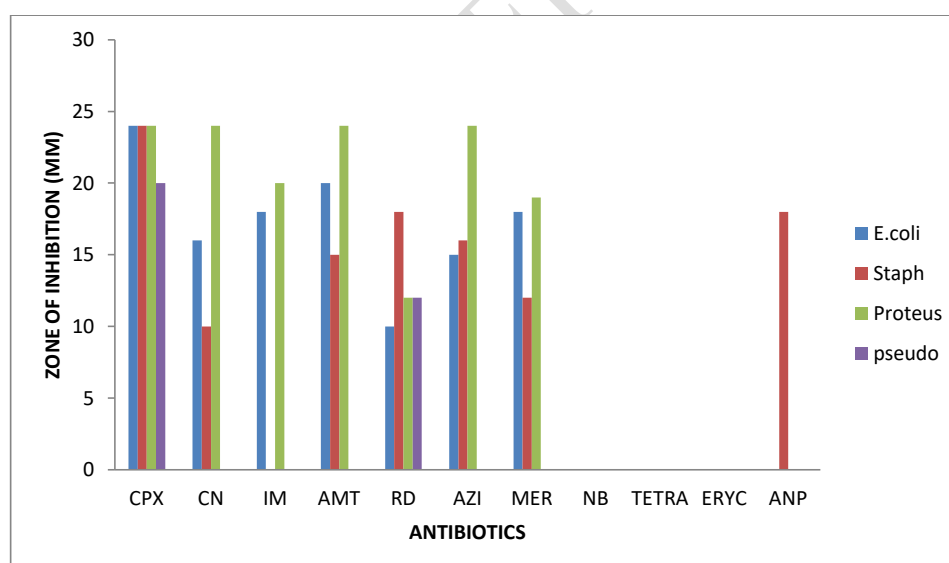
Figure 2: A bar chart with the zone of inhibition (mm) of the antibiotics against to the isolated pathogens.
