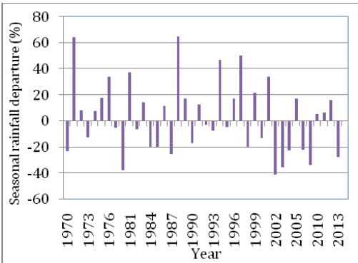
Fig.5: Seasonal rainfall departure at Damoh
