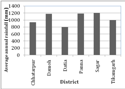
Fig.2. Average annual rainfall in Bundelkhand region (M.P)
