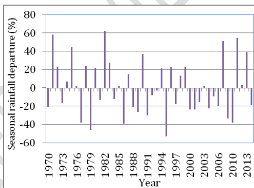
Fig.9: Seasonal rainfall departure at Tikamgarh
