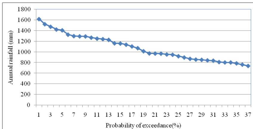
Fig. 11: Probability distribution of annual rainfall at Tikamgarh
