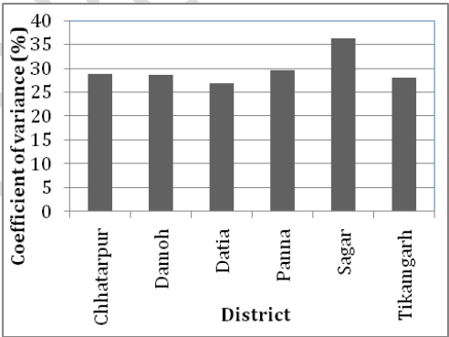
Fig.3. coefficient of variance of annual rainfall
