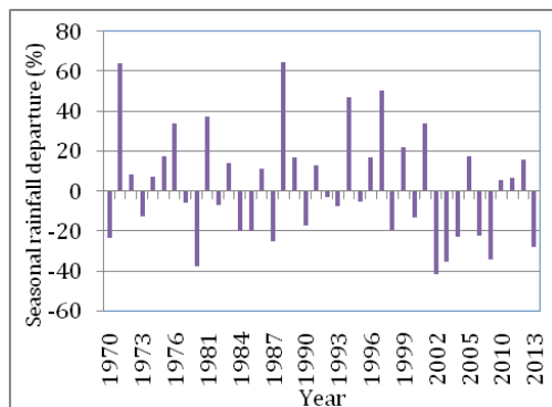
Fig.6: Seasonal rainfall departure at Datia
