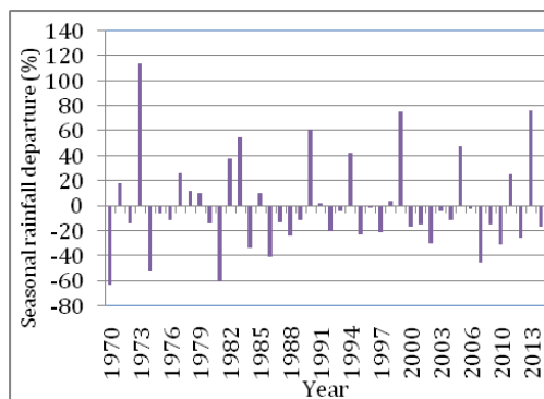
Fig.8: Seasonal rainfall departure at Sagar
