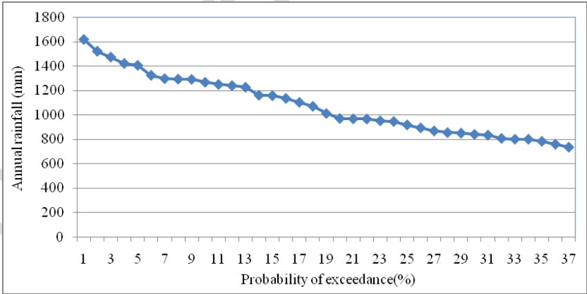
Fig. 10: Probability distribution of annual rainfall at Sagar
