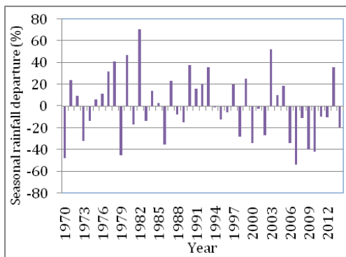
Fig.7: Seasonal rainfall departure at Panna
