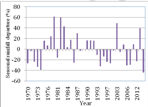
Fig.4: Seasonal rainfall departure at Chhatarpur
