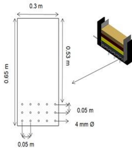
Fig. 12 Dimensions of inner plate in the outlet collection tank
