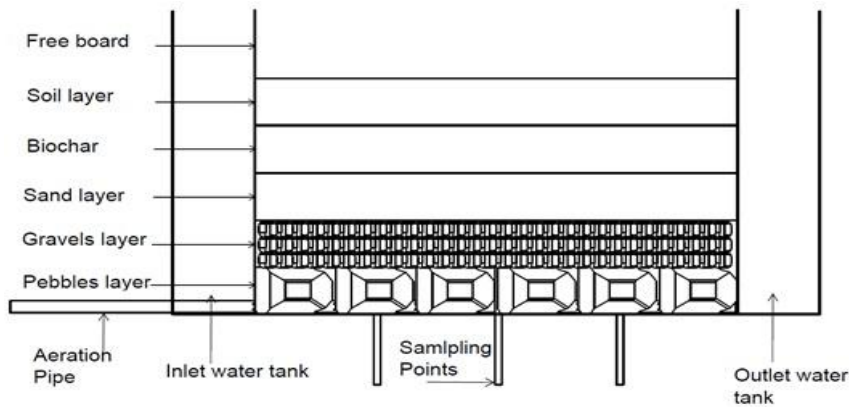
Fig. 5. Schematic diagram of laboratory scale constructed wetland system
