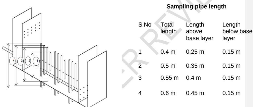
Fig. 3. Isometric view of the different sampling points to collect samples from different layers in laboratory scale constructed wetland system
