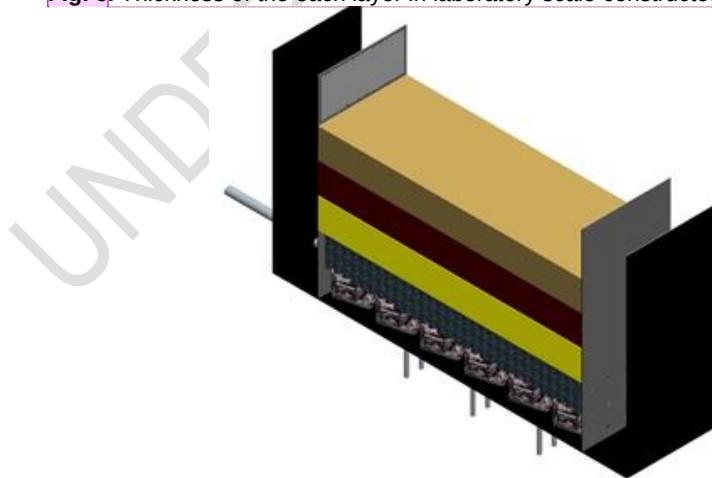
Fig. 7. Isometric view of the each layer in laboratory scale constructed wetland system
