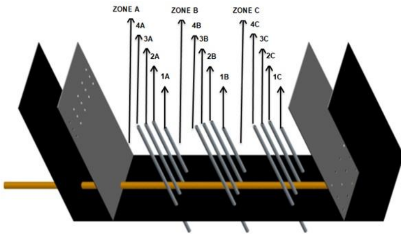
Fig. 13 Sampling collection pipe zone
