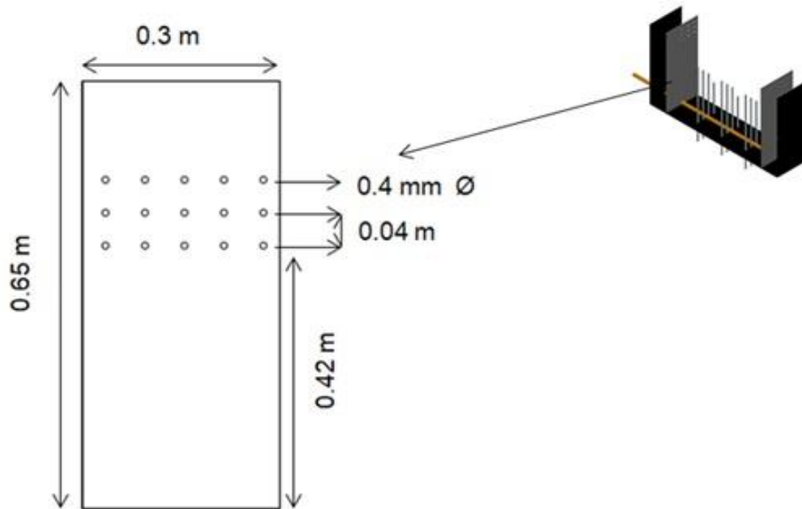
Fig. 8. Dimensions of inner plate in the Inlet collection tank
