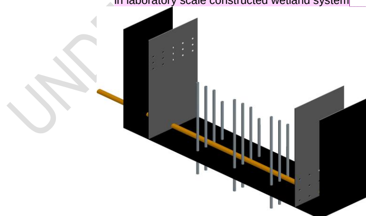
Fig. 4. Digital isometric view of the different sampling points to collect samples from different layers in laboratory scale constructed wetland system
