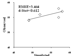
Fig. 2(a): Observed and simulated PI stage of Mahsuri
