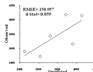
Fig. 2(l): Observed and simulated Grain yield of TTB-404
