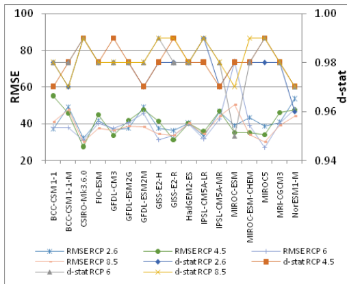
Fig. 1(c): Monthly accumulated Rainfall ( \text{mm month}^{-1} )
