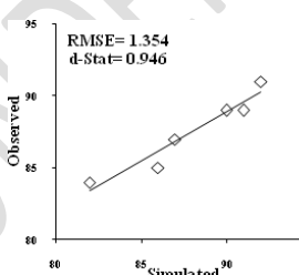
Fig. 2(j): Observed and simulated anthesis stage of TTB-404
