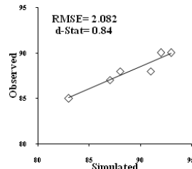
Fig. 2(b): Observed and simulated anthesis stage of Mahsuri
