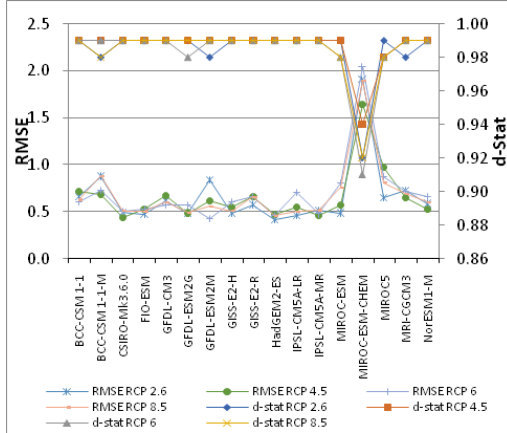
Fig. 1(a): Monthly mean Maximum temperature ( ^{\circ}\text{C month}^{-1} )
