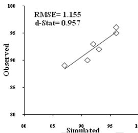
Fig. 2(f): Observed and simulated anthesis stage of Swarna Sub-1
