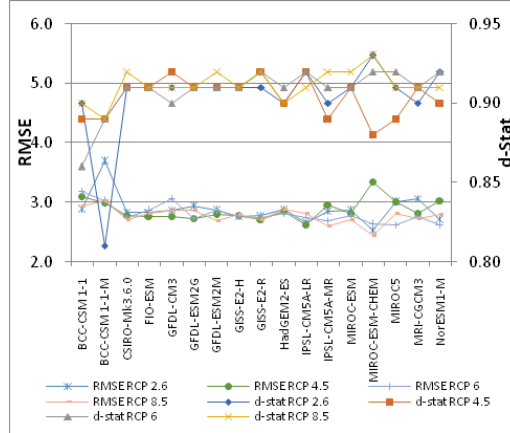
Fig. 1(b): Monthly mean Minimum temperature ( ^{\circ}\text{C month}^{-1} )
