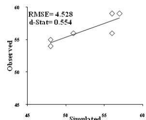
Fig. 2(i): Observed and simulated PI stage of TTB-404
