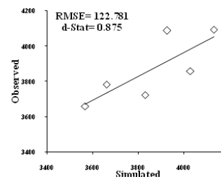
Fig. 2(h): Observed and simulated Grain yield of Swarna Sub-1
