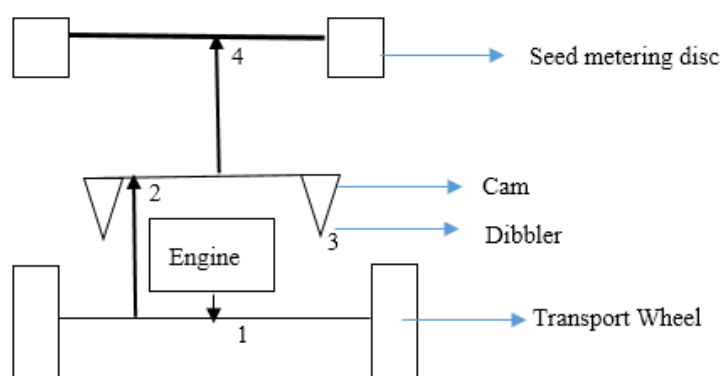
Figure.3 Power transmission diagram
