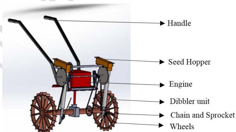
Figure.1 CAD Design – Dibbler
