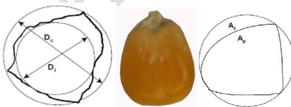
Image.2. Measurement of Sphericity and Roundness
