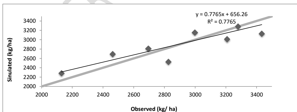
Fig: 3 Relationship between simulated grain yield (kg/ha.) at the harvest of wheat cultivars.
