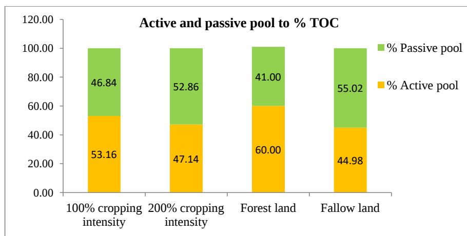
Fig 3. Distribution of active and passive pools up to 0-30cm depth (as % of TOC) under different land use patterns.
