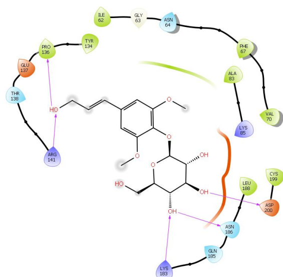
Fig 15: Binding pose of Lilacin with human GSK3β
