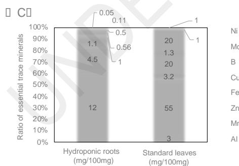
Fig. 1. Ingredient composition in tea roots cultivated hydroponically
