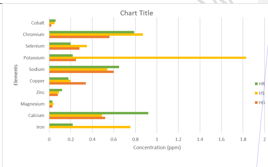
FIGURE 1 Analysis of elemental composition of Hibiscus cannabinus L, Hibiscus acetosella Welw and Hibiscus sabdariffa L.
