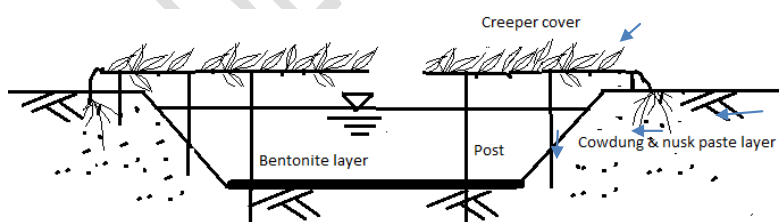
Fig.10 Section of pond with bentonite bottom and top covered by creepers
