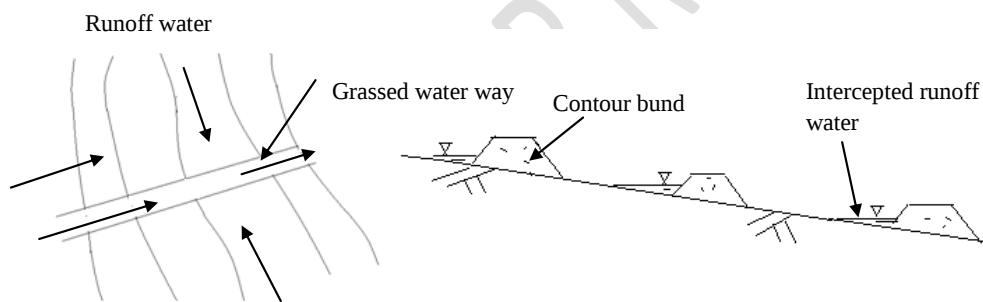
Fig.3 Contour bunds & grassed disposal channel
