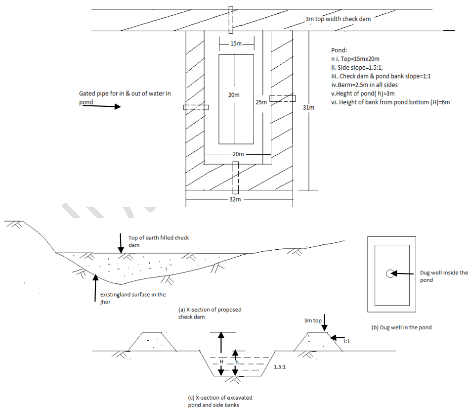
Fig.2 Check dam, ponds & dug-well sections & locations
