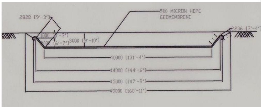
Fig.9 Design section of farm pond
