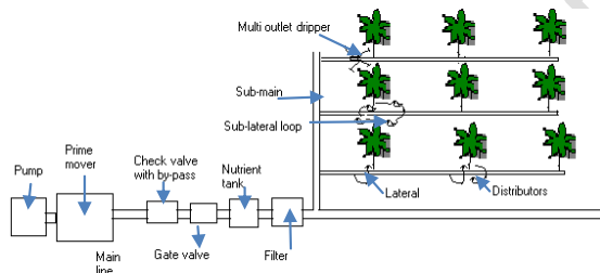
Fig.7 A schematic diagram of drip irrigation system
