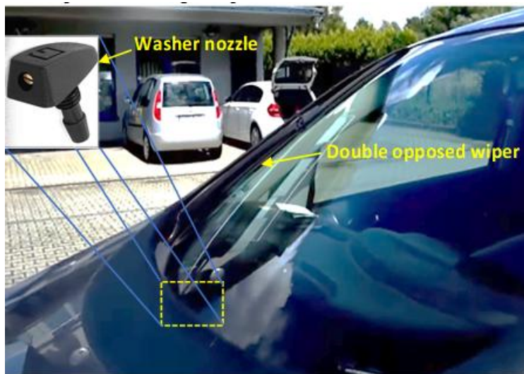
Fig. 14. Horizontally parked wipers of SEAT Altea [15]
