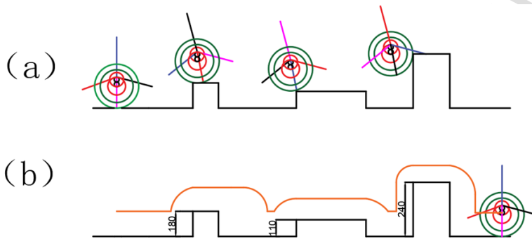
Fig. 6. Simulation results of wheel gait
