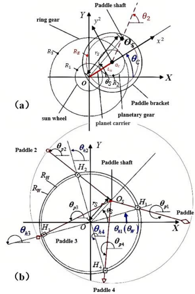
Fig. 4. Schematic diagram of wheel foot movement
