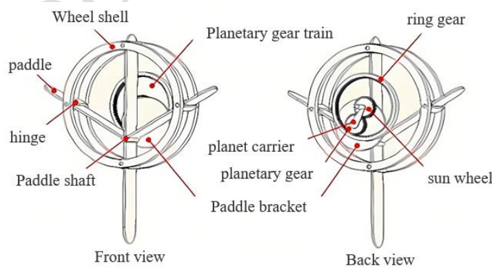
Fig. 3. Schematic diagram of wheel foot structure
