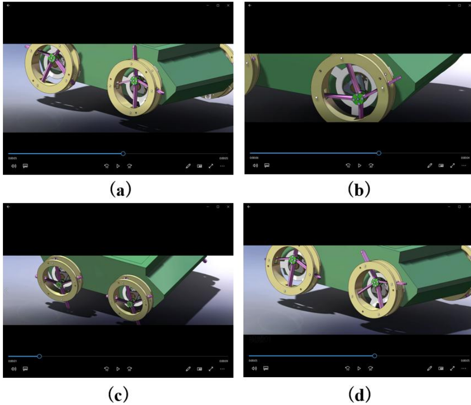
Fig. 11. animation demonstration of four gaits
