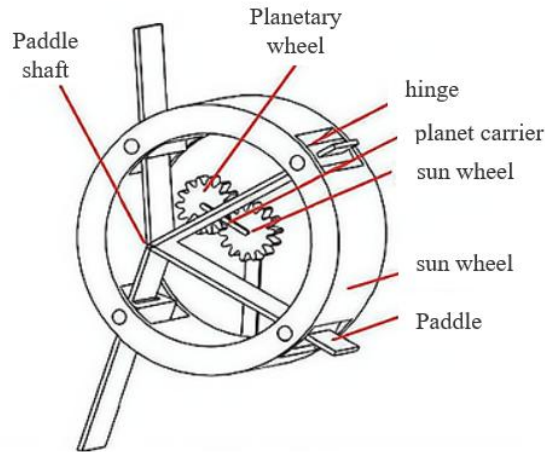
Fig. 1. schematic diagram of e paddle structure
