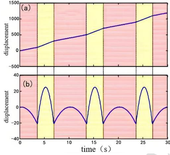
Fig. 9. Relative displacement of propeller shaft
