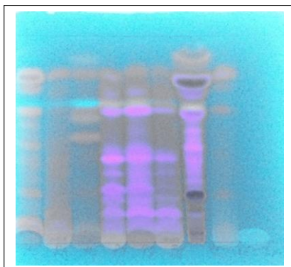
Figure 9. Chromatogram for alkaloids [Mobile phase: Toluene/ethyl acetate/diethylamine (35: 10: 5); Detection: \text{NaNO}_2 5%]. Alkaloids are characterized by the presence of orange
