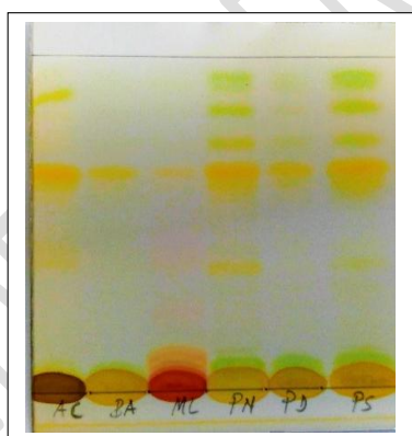
Figure 9. Chromatogram for alkaloids [Mobile phase: Toluene/ethyl acetate/diethylamine (35: 10: 5); Detection: \text{NaNO}_2 5%]. Alkaloids are characterized by the presence of orange
