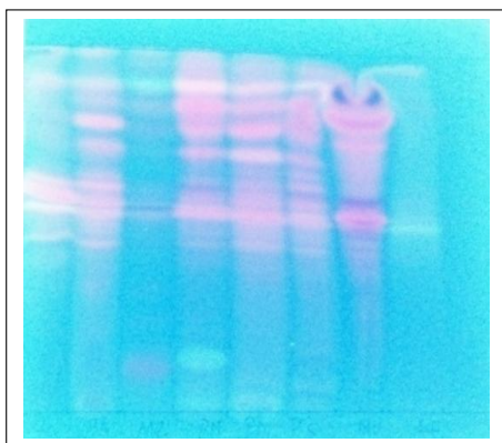
Figure11. Chromatogram of the methanolic extract of A. cordifolia , B. alba , M. lucida , P. nigrescens , P. dodecandra and P. scandens for anthraquinones; Mobile phase: Ethyl acetate/Methanol/Water (50: 8.5: 6.5). Detection: by UV light at 366 nm.
