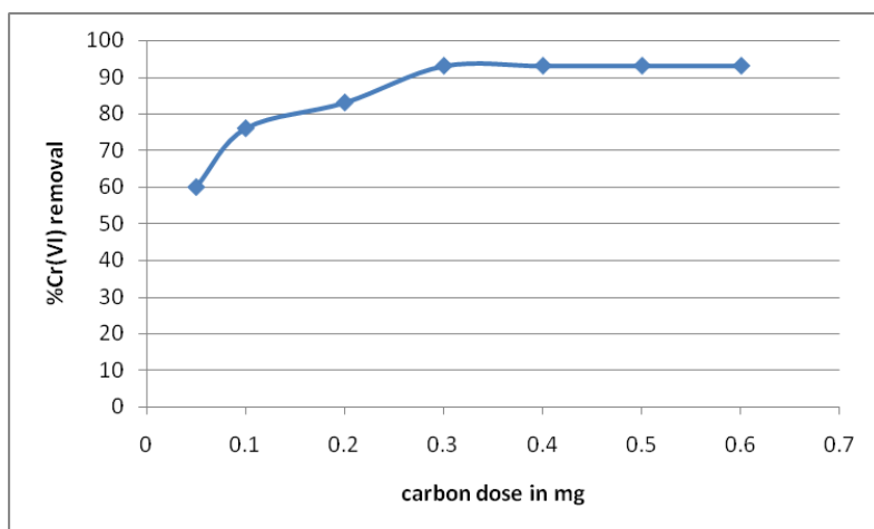
Figure 2. Effect of carbon dose on Cr(VI) removal
