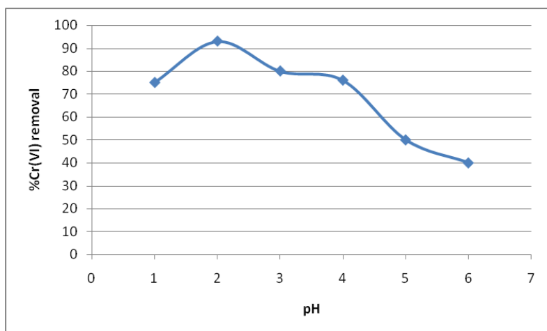
Figure 1. Effect of pH on Cr(VI) removal
