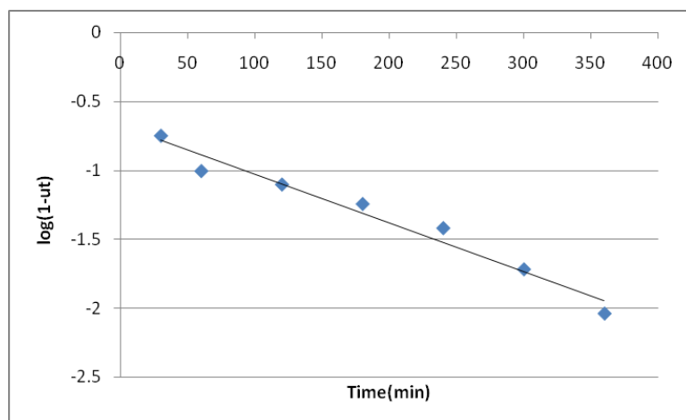
Figure 4 Reversible first order kinetics for Cr(VI) removal
