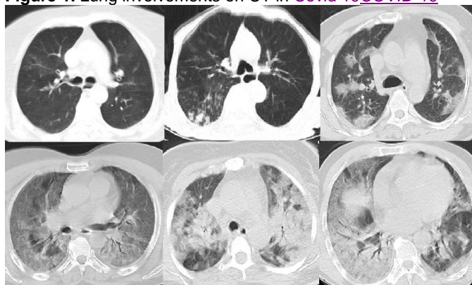
Figure 1. Lung involvements on CT in Covid 19 COVID-19
