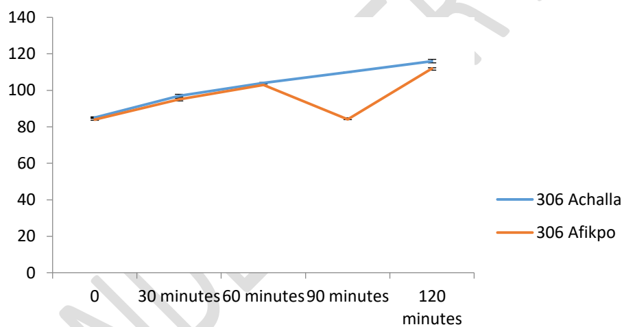
Fig. 2. Graph of glycemic responses after feeding on 306
