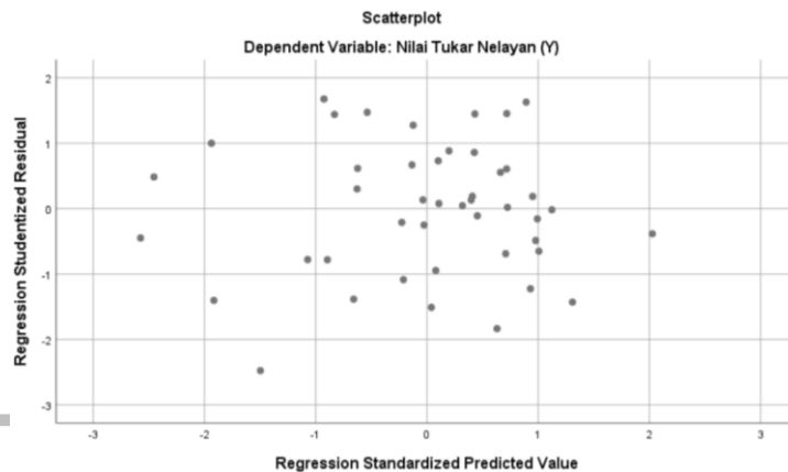
Fig 2. Fisher heteroscedasticity
