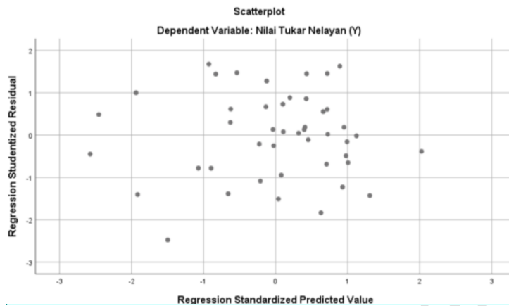
Fig 2. Fisher heteroscedasticity
