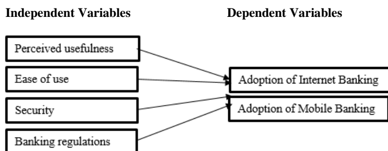
Figure 1 Conceptual Framework
