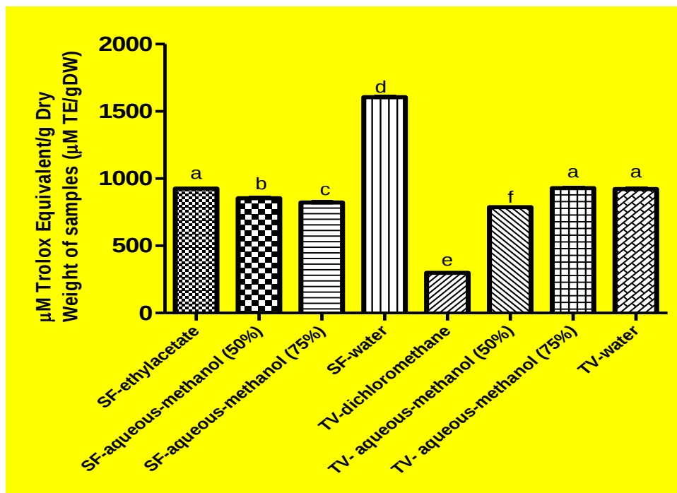
Figure 3: Trolox equivalent absorbance capacities of S. frutescens and T. violacea extracts. Data are expressed as mean \pm SEM of triplicate samples. Bars with the same superscript are not statistically different at P=.05 .
