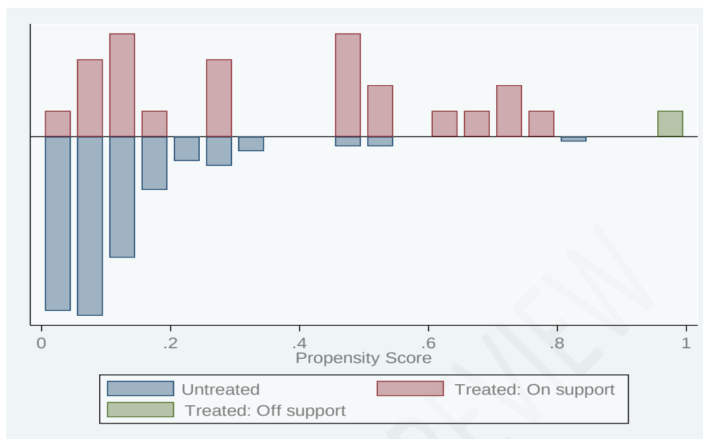
Figure 1: Propensity scores distribution
