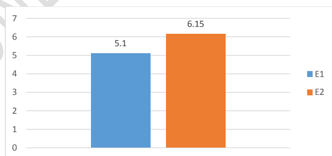
Fig. 1. Evolution of the electric conductivity from the water used for the maize cooking process (E1) to solutions from maize cooking (E2)
