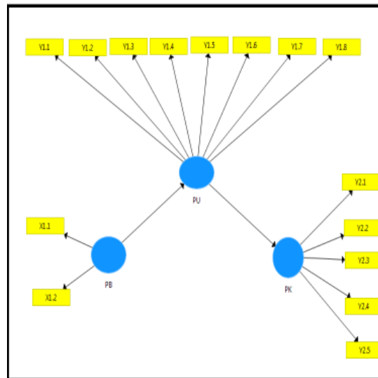
Picture. 2 Outer Model
