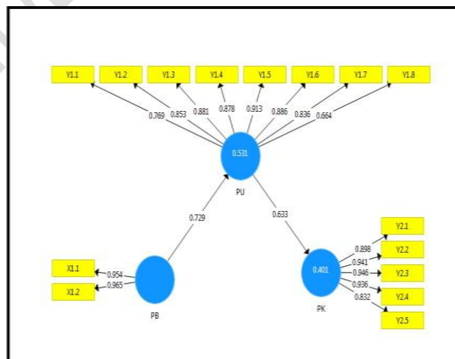
Picture. 3 Convergent Validity Test
